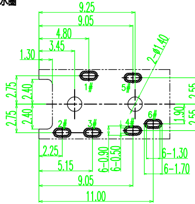
P.C.B LAYOU T=1.00mm TOP VIEW
