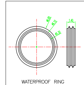
WATERPROOF RING
