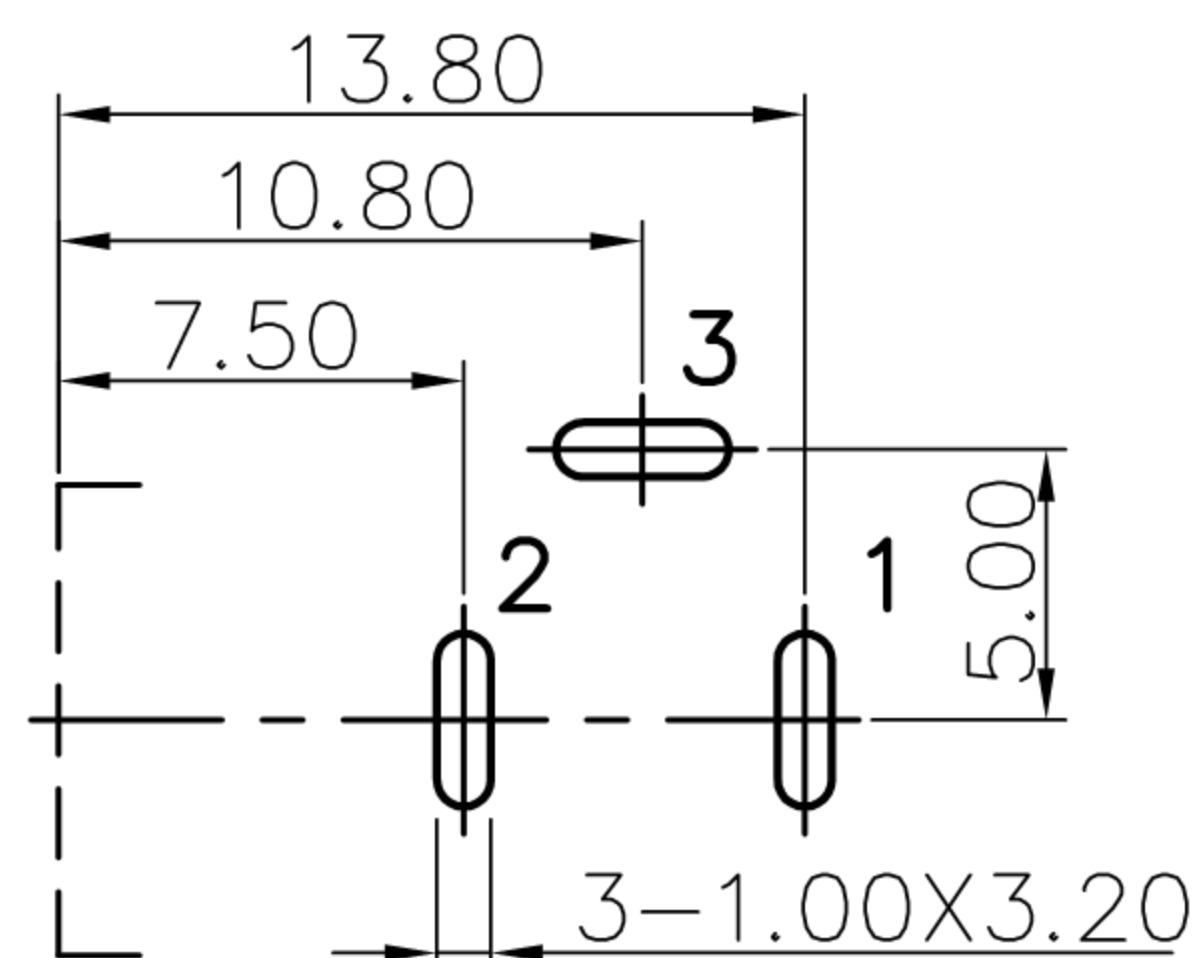
Pin Hole Layout (Jack Bottom View)
