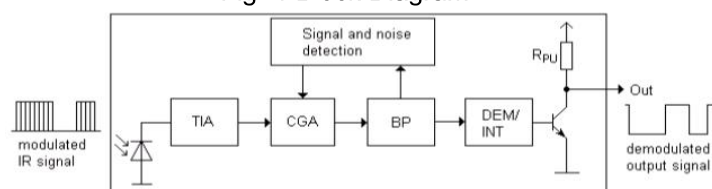
Fig.-1 Block Diagram
