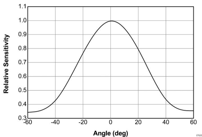
Fig.5 Relative Sensitivity vs. Angle
