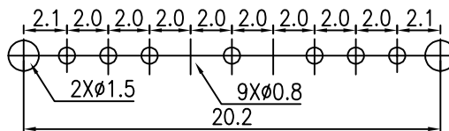
P.C.B LAYOUT TOP VIEW
