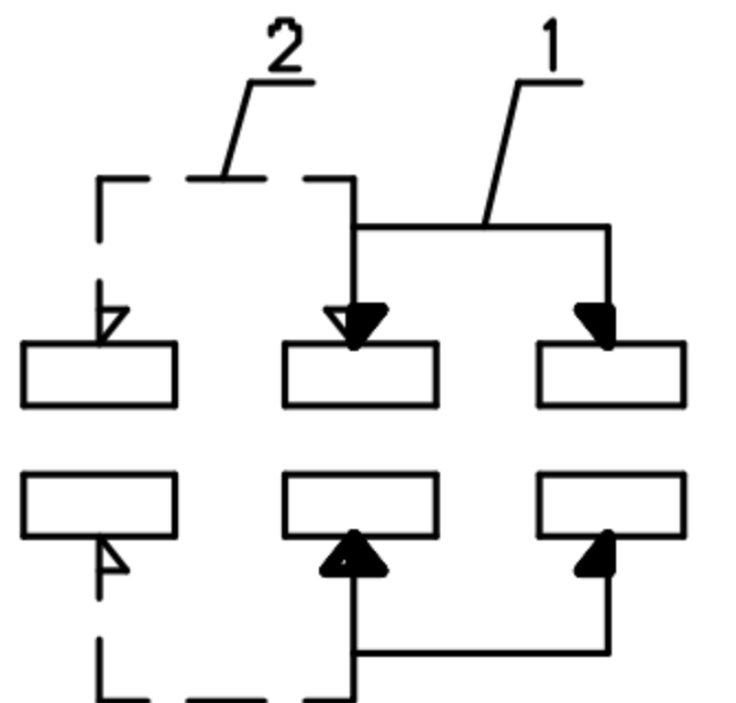
SLIDE SWITCH 2P2T
