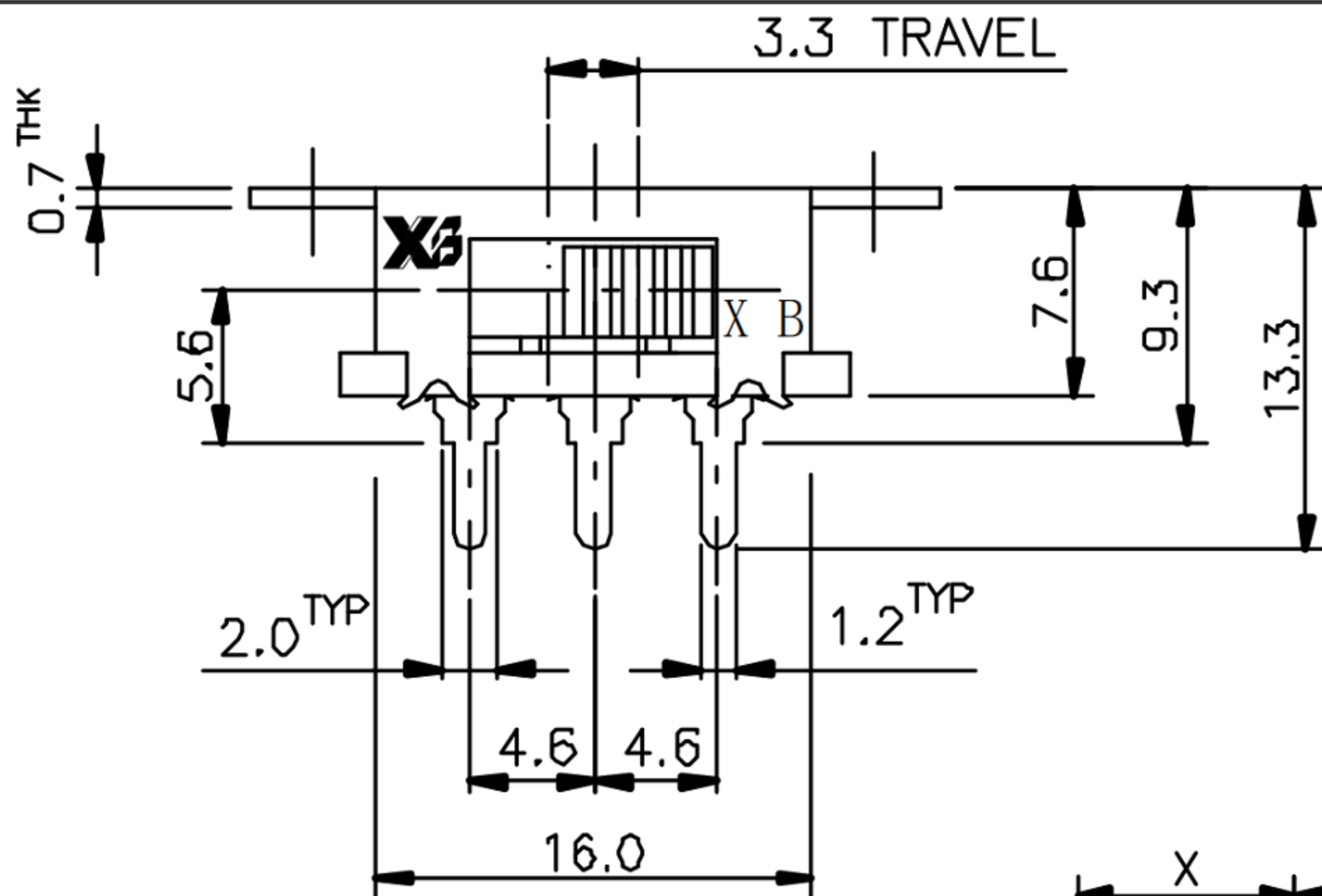
SLIDE SWITCH 2P2T
