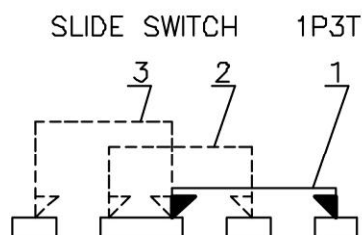
SCHEMATIC (SHORTING)
