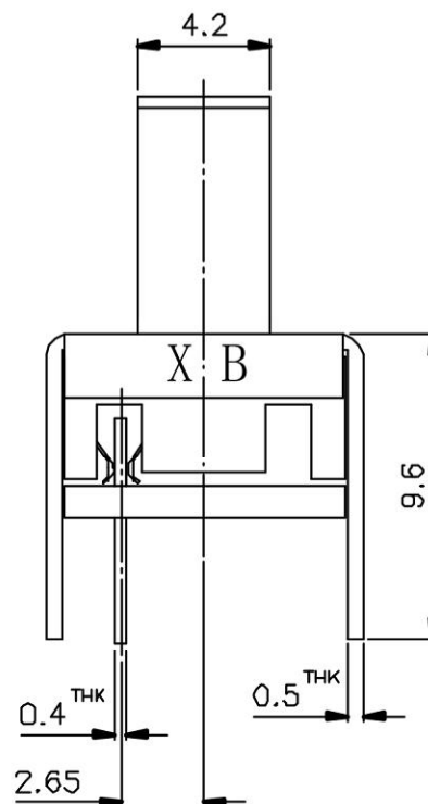
SLIDE SWITCH 1P3T
