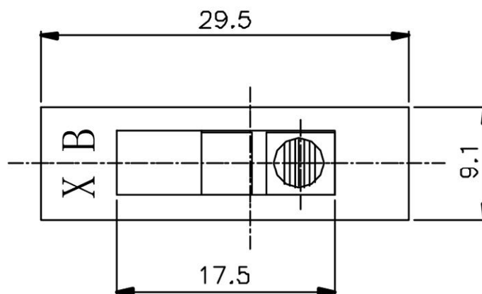
SLIDE SWITCH 2P4T
