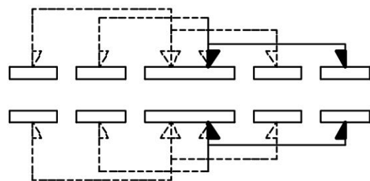
NON-SHORTING SCHEMATIC
