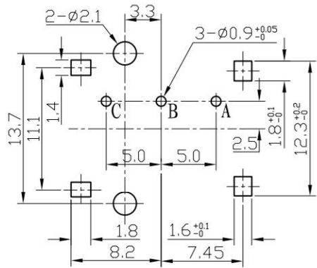
GENERAL TOLERANCES: \pm 0.05 P.C.B MOUNTING
