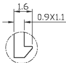
VIEW I 2 : 1
