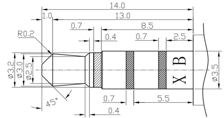
MATE PLUG
