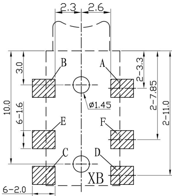
P. C. B LAYOUT
