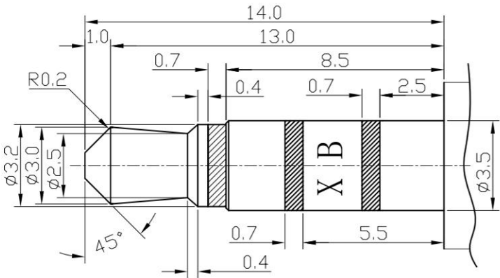
MATE PLUG
