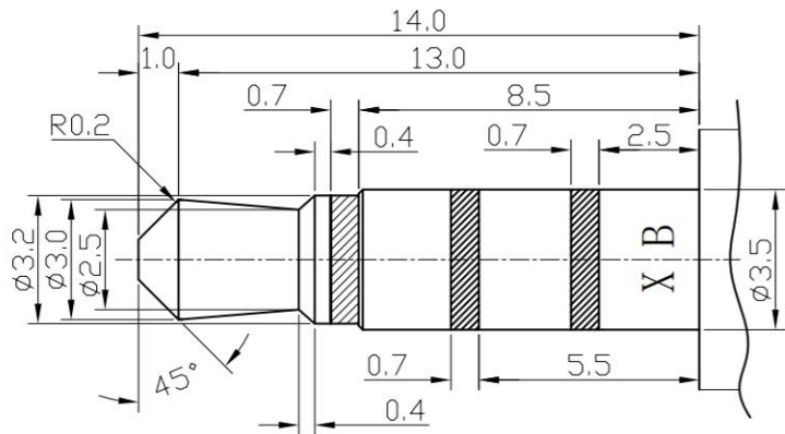
MATE PLUG
