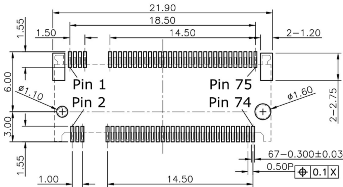
Recommended Layout (Top View) General Tolerance: ±0.05mm
