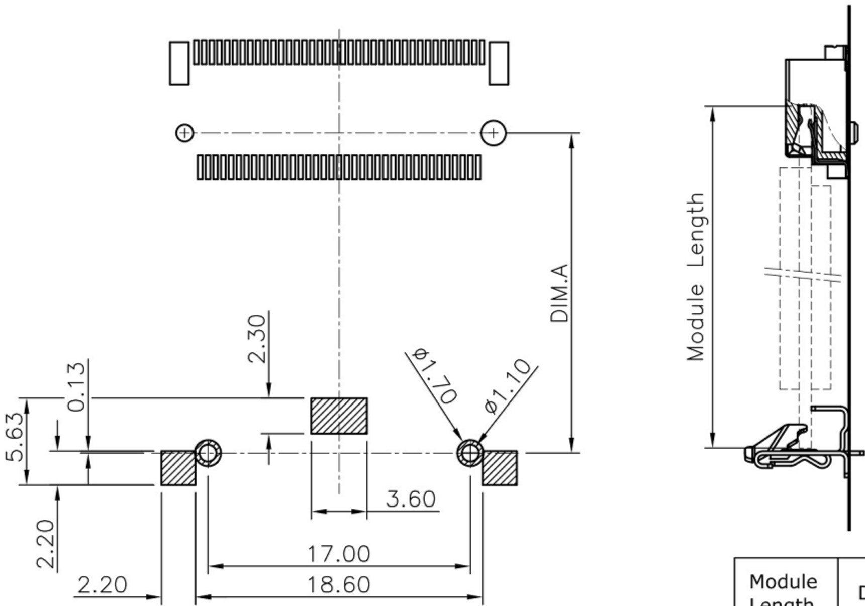
RECOMMENDED LAYOUT (TOP VIEW) GENERAL TOLERANCE: ±0.05mm
