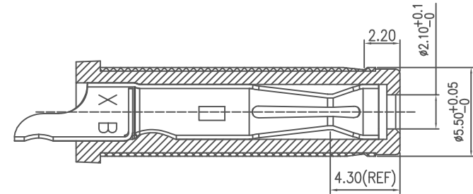
MATING PLUG
