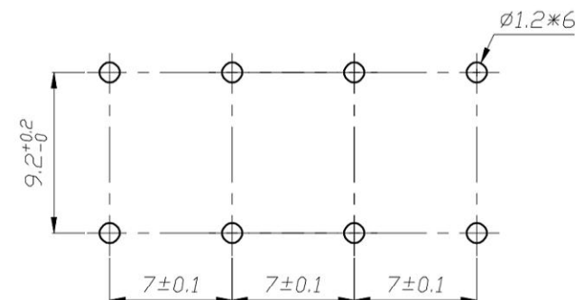
PCB MOUNTING HOLE ARRANGEMENT
