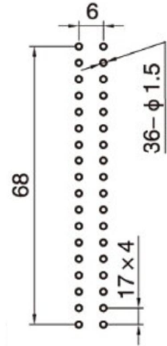
PCB LAYOUT
