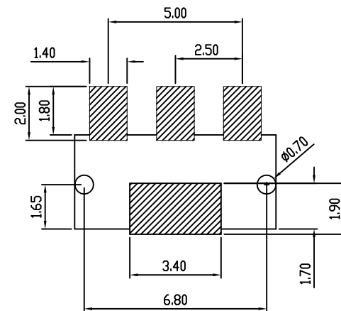
RECOMMENDED PCB LAYOUT TOL: (<math>\pm 0.05</math>)
