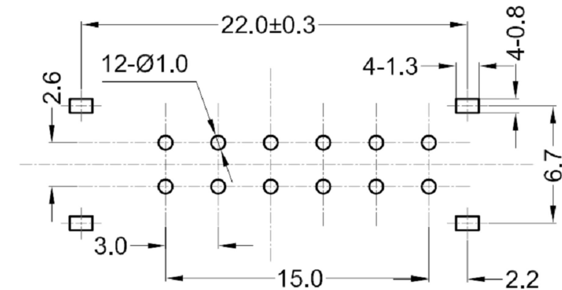
P.C.B LAYOUT BOTTOM VIEW
