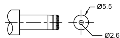
MATING PLUG Jack Insertion Depth: 9.15 mm
