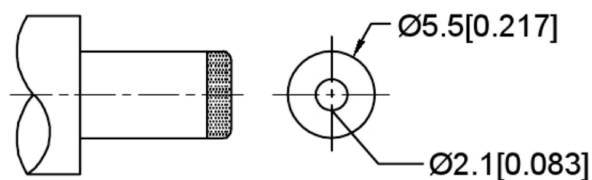
MATING PLUG Jack Insertion Depth: 9.0 mm
