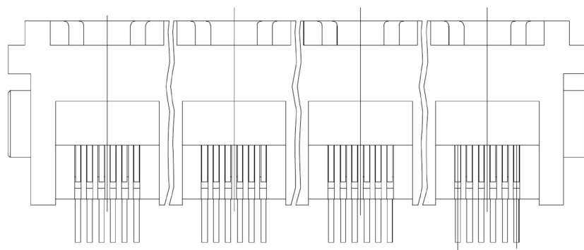
BOTTOM VIEW
